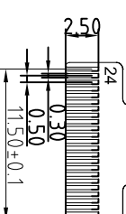
BOTTEM VIEW
